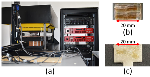
Fig. 2. (a) Open-sided ASELSAN FFL scanner. (b) A cylindrical phantom with two parallel tubes was filled with Perimag MNPs at a dilution of 1:20. (c) A Y-shape phantom was filled with Perimag at a dilution of 1:100 and contained a central air bubble.
