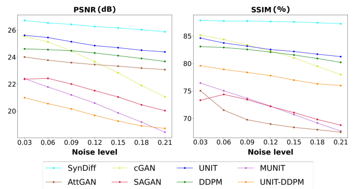
Fig. 6. Performance of competing methods as a function of added noise level on source-modality images. Results shown for the representative T_2 \rightarrow CT task in terms of PSNR (left), SSIM (right).
